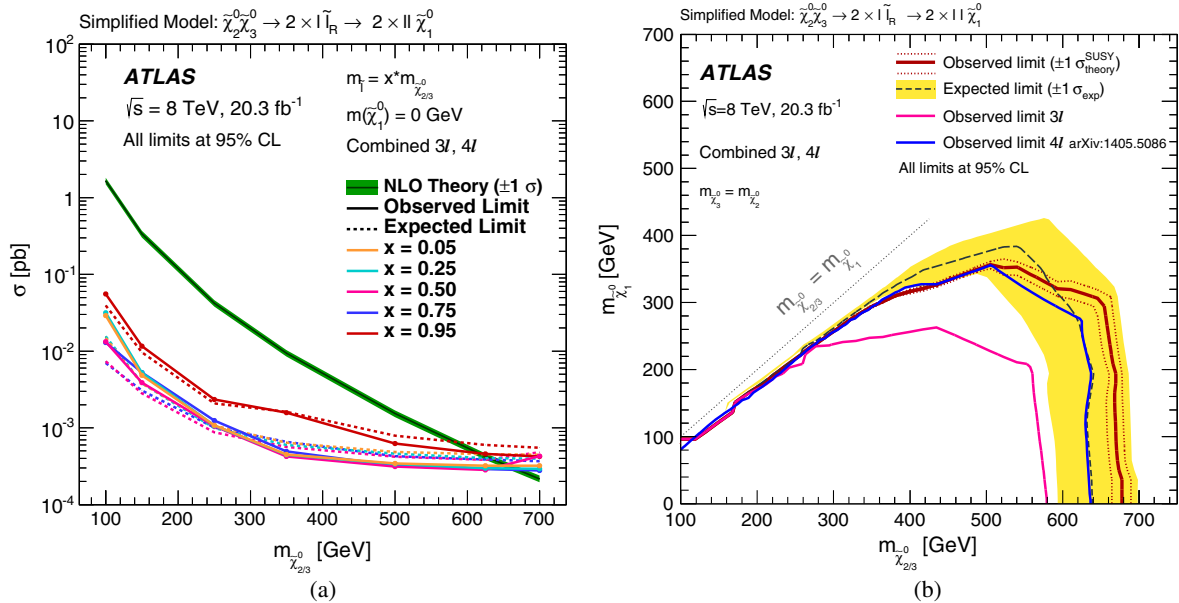
FIG. 15. The 95% CL exclusion limits on \tilde{\chi}_2^0\tilde{\chi}_3^0 production with \ell_R -mediated decays, (a) where the \tilde{\chi}_1^0 is massless and the intermediate slepton mass is set to 5%, 25%, 50%, 75%, and 95% of the \tilde{\chi}_2^0 mass, and (b) as a function of the \tilde{\chi}_2^0 and \tilde{\chi}_1^0 masses, where the slepton mass is halfway between the \tilde{\chi}_2^0 and \tilde{\chi}_1^0 masses. The limits in (a) and (b) are set using a combination of the 3\ell analysis from Ref. [20] and the 4\ell analysis from Ref. [21].
