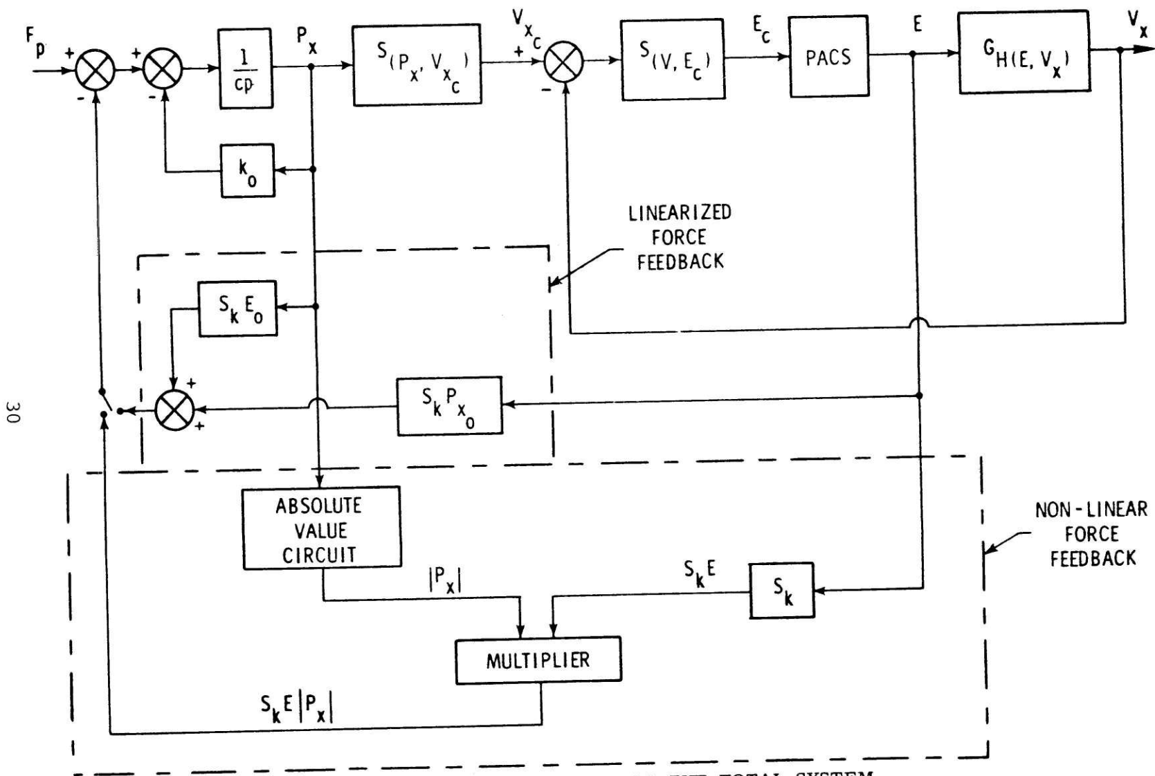
SCHMATIC ILLUSTRATION OF THE TOTAL SYSTEM FIGURE 3.2
