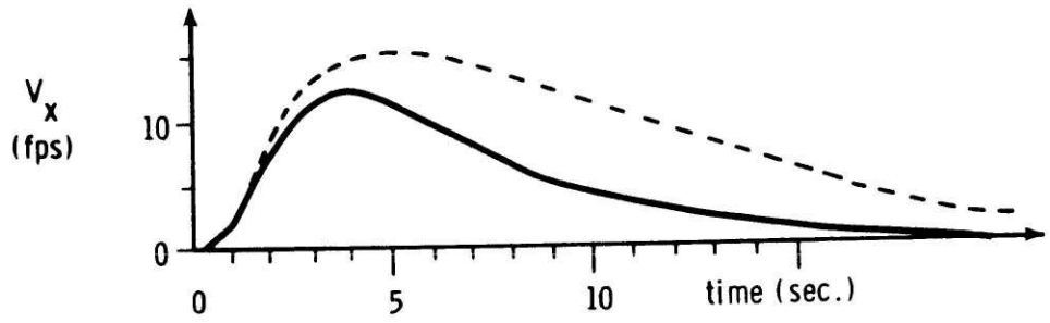
TIME RESPONSE OF THE IDEALIZED SYSTEMS FIGURE 2.5
