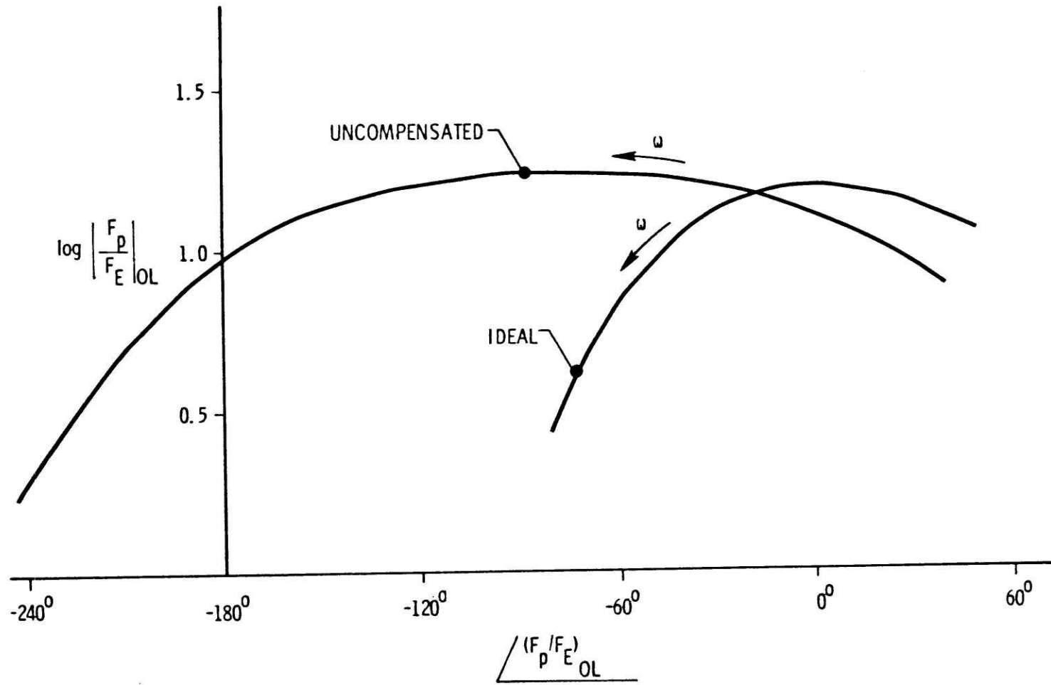
NICHOLS CHART FOR THE LINEARIZED SYSTEMS
