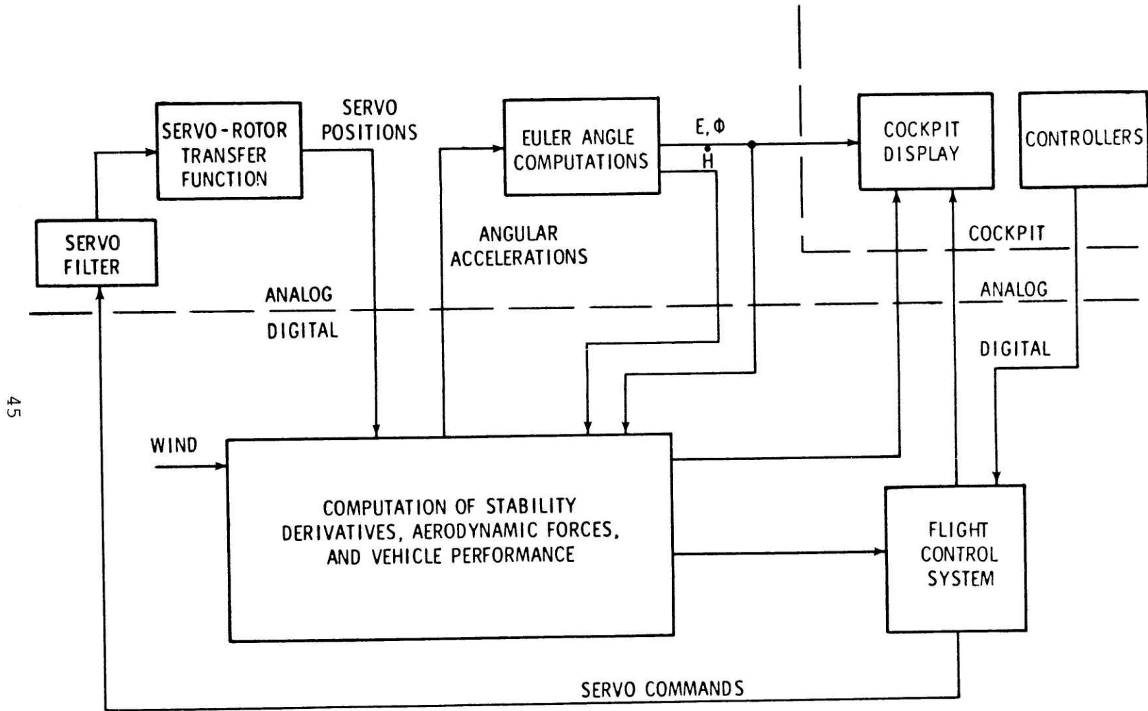
SCHEMATIC REPRESENTATION OF THE TEST INSTALLATION
