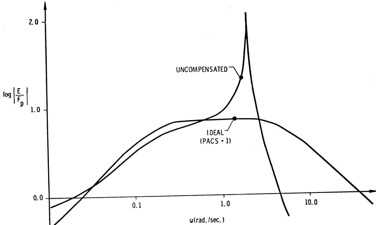
BODE GAIN DIAGRAMS OF THE LINEARIZED SYSTEMS FIGURE 3.4
