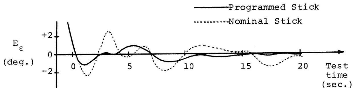
Figure 5.1 Typical Pitch Errors for an Attitude Control Task
