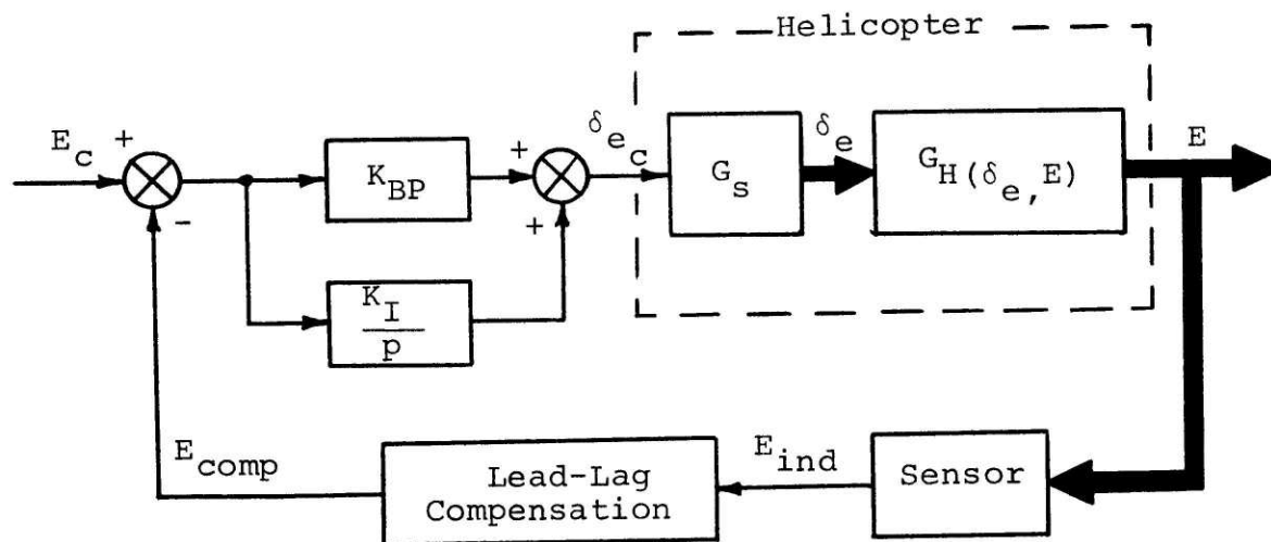
Figure 3.1 Block Diagram of Pitch Attitude Control System
