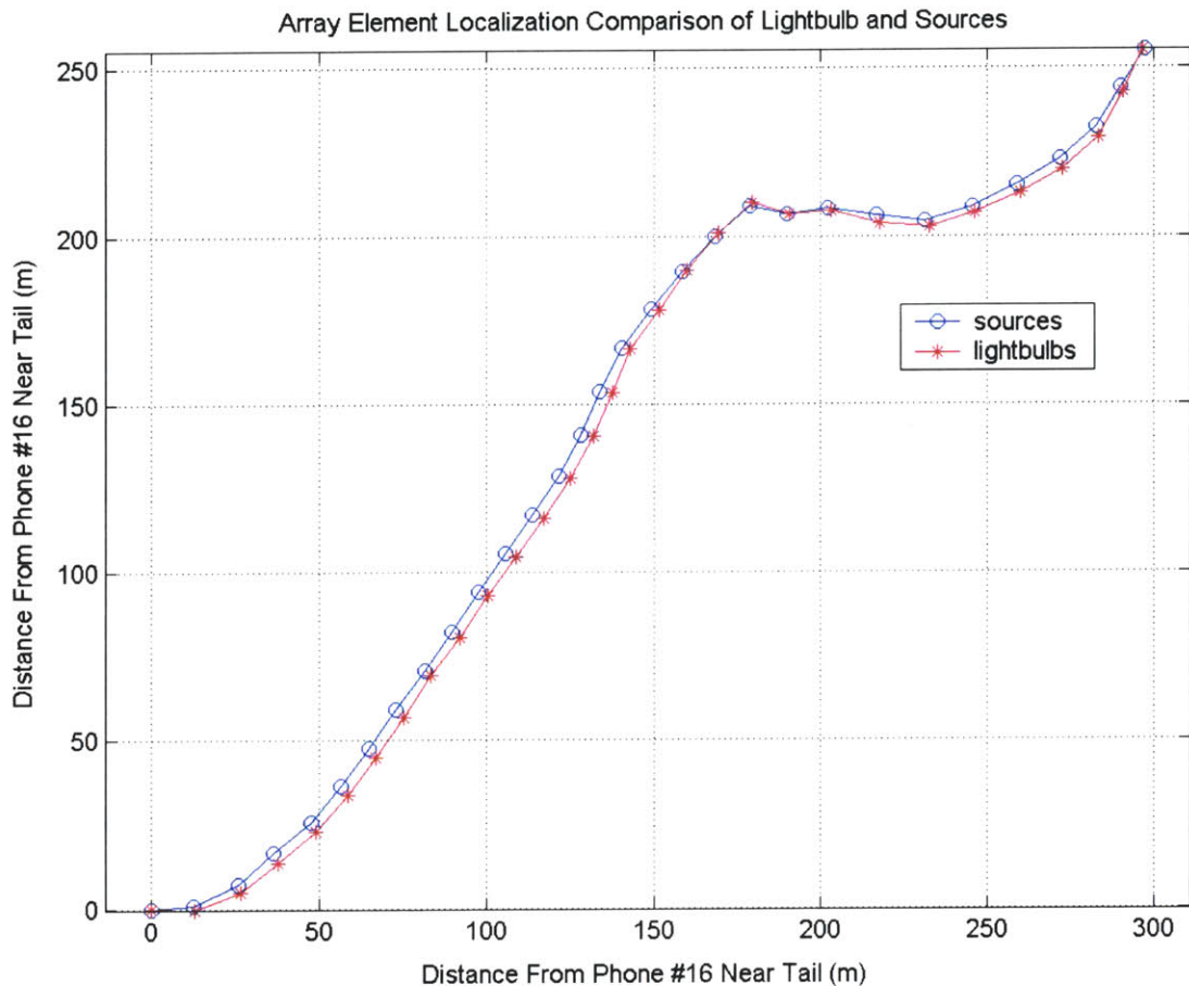
Figure 5-1: Comparison of HLA sensor positions obtained from the distant low frequency moored sources and the light bulb drops. The axes are in meters from the position of hydrophone 16 (closest to the tail).
