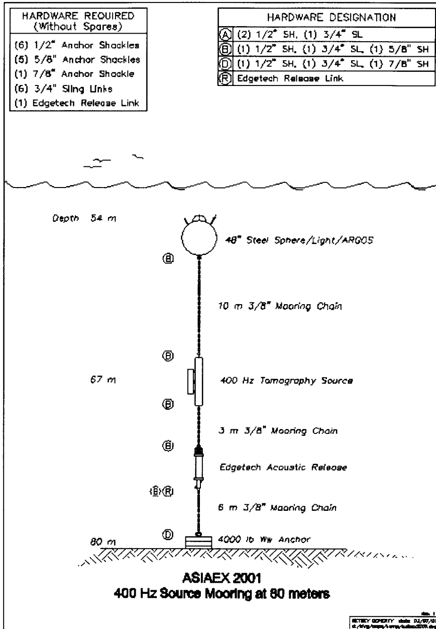
Figure 2-4: Mooring configuration for the 400 Hz sources. Both the deep and shallow sources had the same configuration. The shallow source was actually deployed at 112.7 m depth and the deep source was at 342.5 m water depth.
