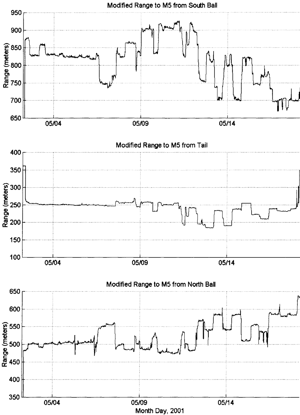
Figure 3-5: Ranges from transponders to LBL channel M5 using the correction in Table 3-1 to correct for changes between direct and surface bounce propagation.
