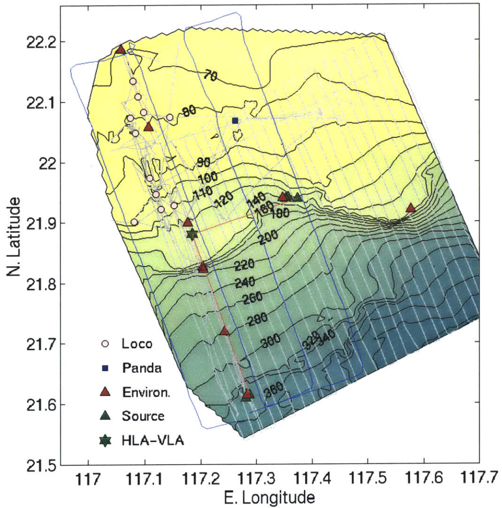
Figure 2-11: Bottom contours for the ASIAEX SCS experiment. The gray lines are the tracks of the research vessels used to interpolate the bottom contours.
