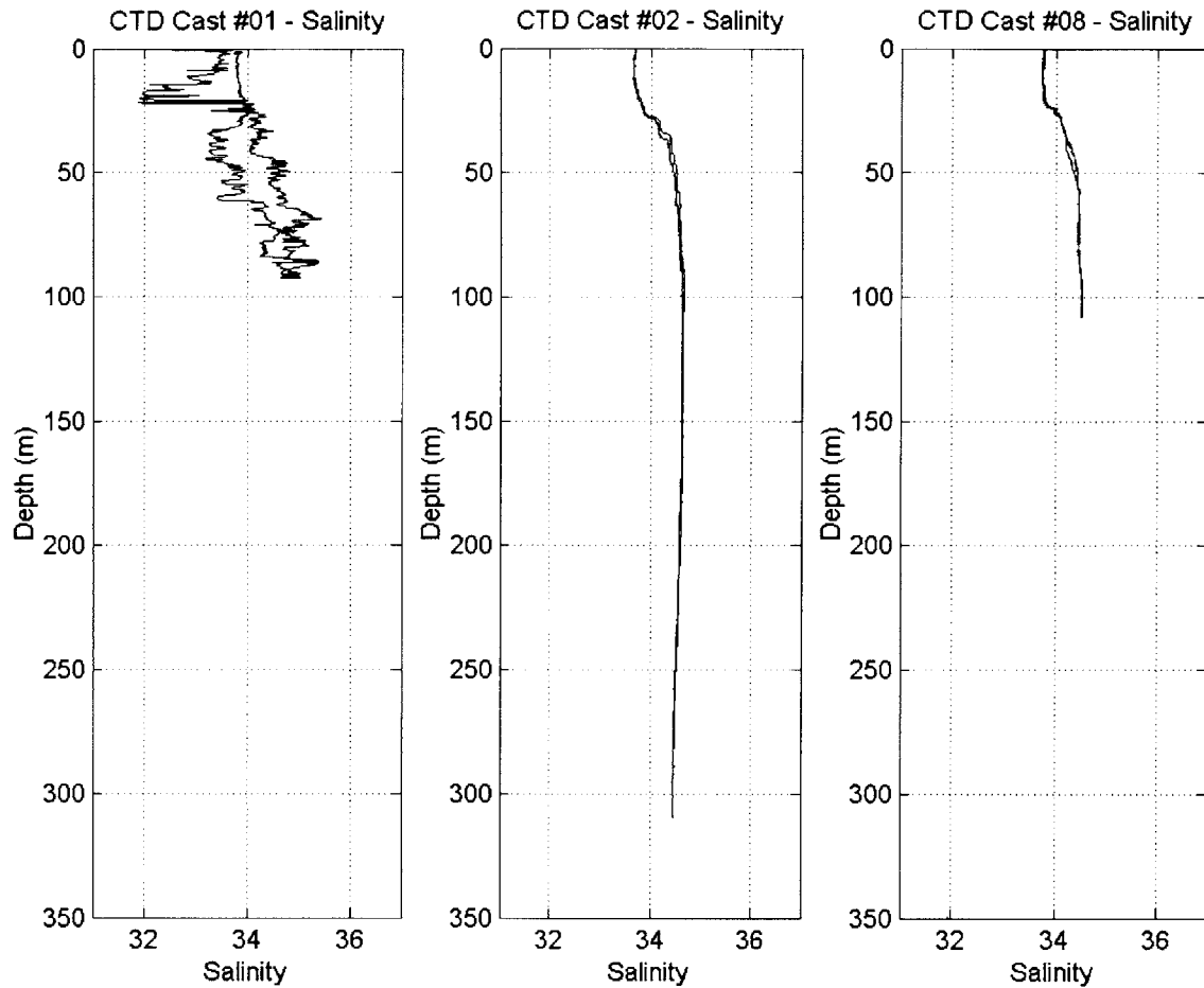
Figure 2-7: CTD salinity from: cast 1 (near the shallow acoustic sources), cast 2 (near the deep acoustic sources) and cast 8 (near the VLA/HLA).
