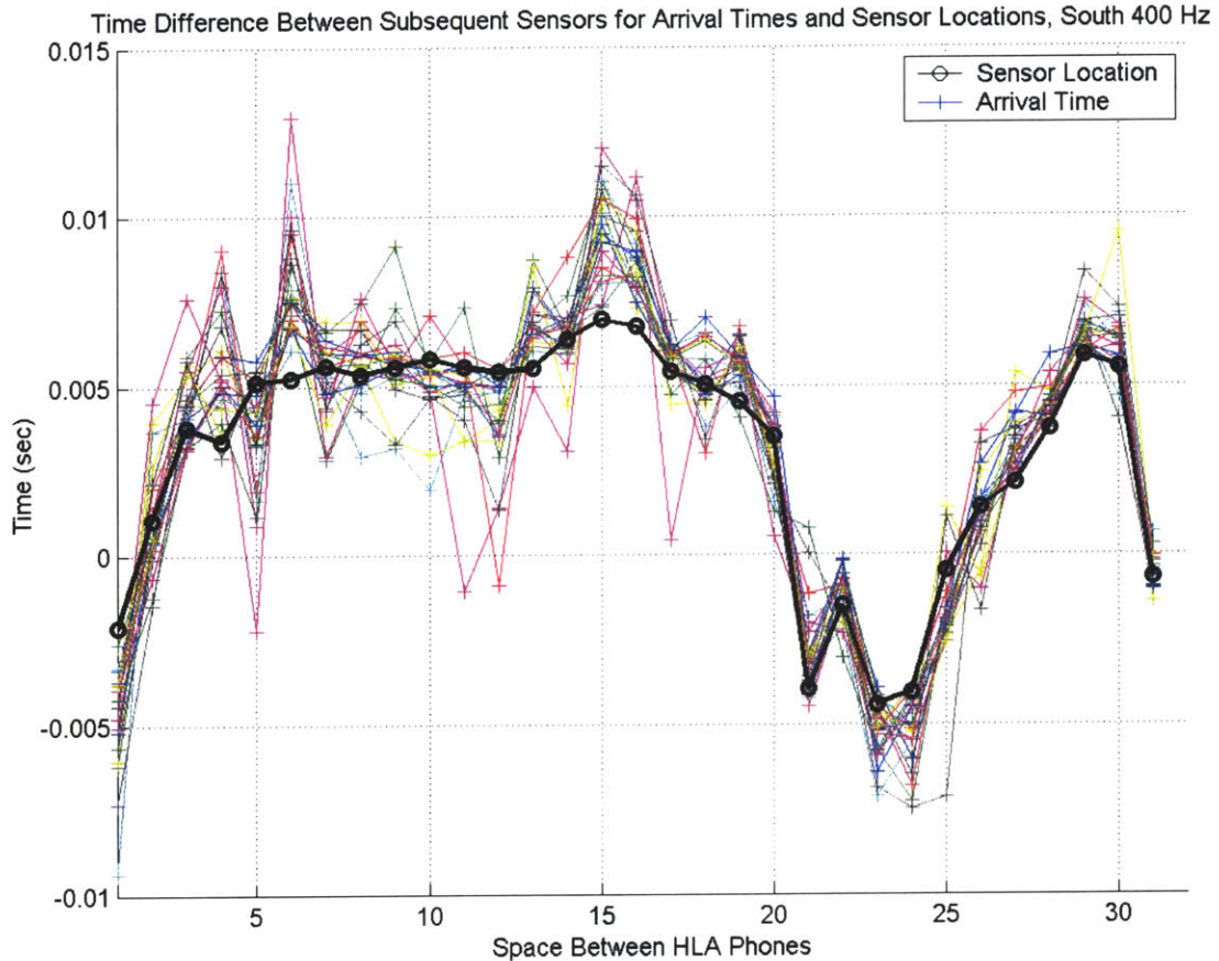
Figure 3-15: Time difference between the arrival times of subsequent hydrophones (space 1 is between Ch16 and Ch17) calculated by taking the difference between the arrival times found from the 400 Hz source transmissions on 5 May. This is compared to the time difference calculated from the sensor locations determined from the light bulb drops on 5 May.
