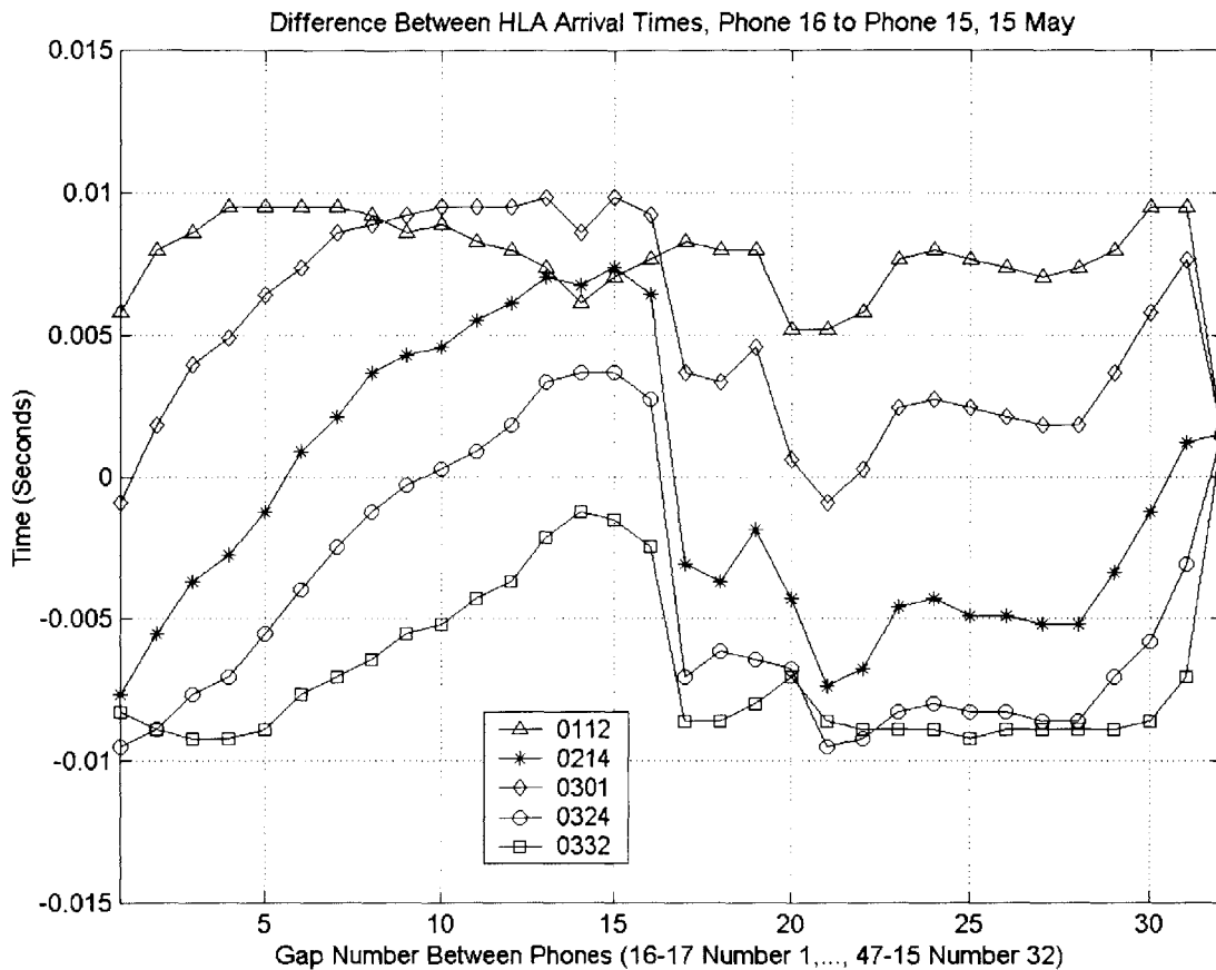
Figure 3-9: Difference between arrival times for successive hydrophones along the HLA, including the time difference between CH47, closest to the sled, and CH15, lowest on the VLA. The x-axis is the number index of the gap between the hydrophones starting with CH16 and CH17, the farthest from the sled. Each of the five drops of 15 May is plotted. The graph verifies good thresholds were used for each drop, as the curves are relatively smooth and none of the time differences exceed .01 seconds, the maximum allowable for the 15 m “fully stretched” sensor spacing.
