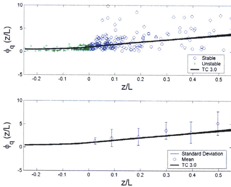
Figure 4.2 Dimensionless Moisture Flux
