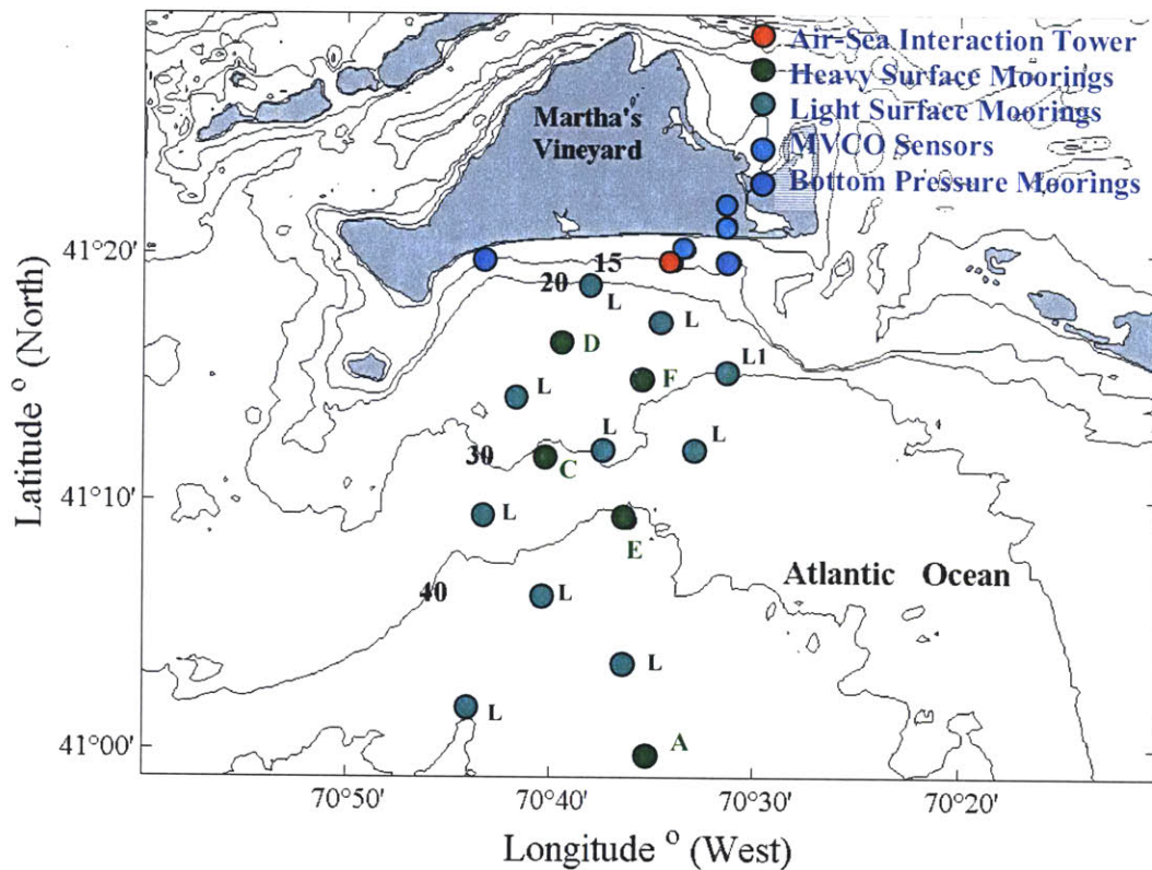
Figure 2.2 CBLAST Offshore Array
