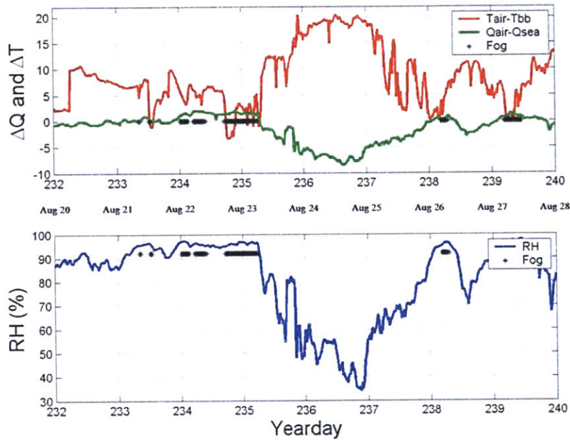
Figure 2.5 Parameters used to identify fog
