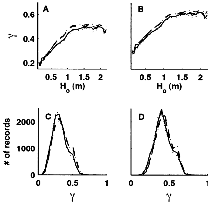
Figure 2-4: The mean best-fit \gamma ( \pm 0.1 m bins in H_o ) versus deep-water wave height H_o at SandyDuck for (A) TG and (B) Bald models for the four different error metrics (solid curve is eqn (2-24), dotted curve is eqn (2-26), dashed curve is eqn (2-27), and dashed-dotted curve is eqn (2-28) and (C & D) the corresponding number of records (i.e., histograms) versus best-fit values of \gamma at SandyDuck.
