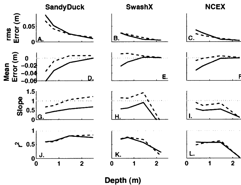
Figure 4-10: (A-C) Root-mean square (rms) and (D-F) mean errors, and (G-I) best-fit slopes and (J-L) correlations ( r^2 ) between the observations and predictions for the LHS model (solid curve) and the full model (dashed curve) for (A, D, G, and J) SandyDuck, (B, E, H, and K) SwashX, and (C, F, I, and L) NCEX versus water depth. The horizontal dotted lines represent either zero (mean errors) or 1 (slope and r^2 values).
