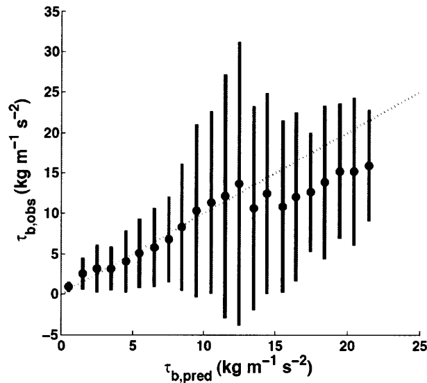
Figure 4-7: Means (circles, 1 \text{kg m}^{-1} \text{s}^{-2} -wide bins) and standard deviations (solid lines) of \tau_{b,obs} calculated from the observed undertow assuming a linear variation with depth and a no-slip bottom boundary condition versus \tau_{b,pred} modeled using (4-15). The dotted line is perfect agreement.
