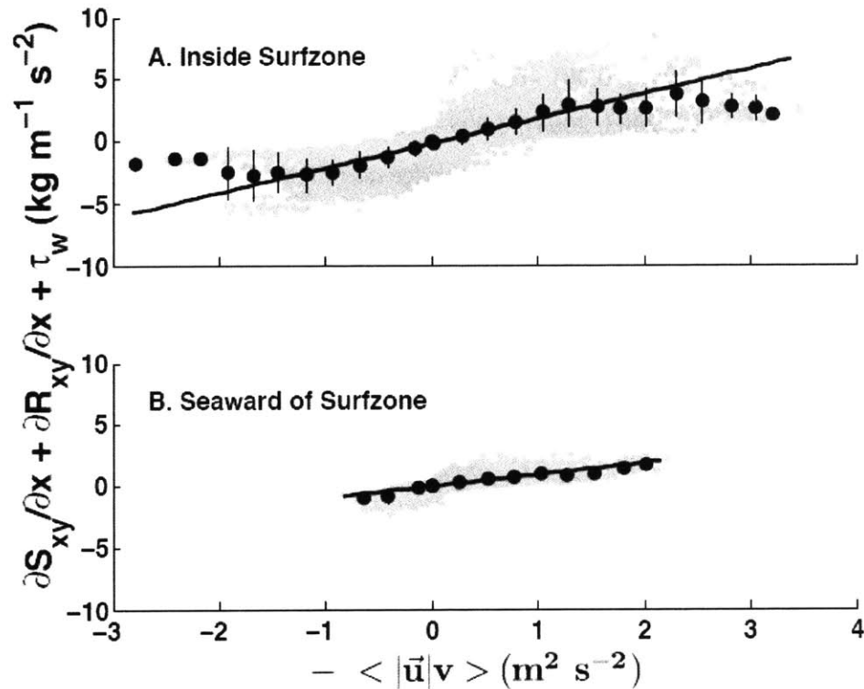
Figure 4-5: The total alongshore forcing ( dS_{xy}/dx + dR_{xy}/dx + \tau_w ) versus the velocity term - \langle |\vec{u}|v \rangle in the bed stress formulation for sensors (A) inside the surfzone and (B) seaward of the surfzone. The light grey dots are the 8.5 min values. Solid circles and vertical hashes are the means ( 0.025\text{-m}^2\text{s}^2 - wide bins) and standard deviations, respectively. The solid lines are the least squares fits to the unbinned values.
