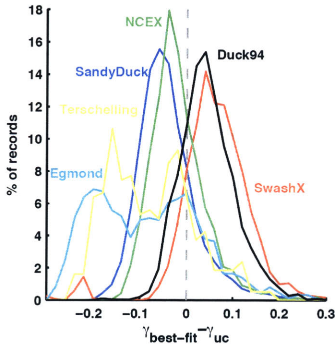
Figure 2-10: Percent of data records for the TG model versus the difference between the best-fit \gamma ( \gamma_{\text{best-fit}} ) and the \gamma based on the universal curves ( \gamma_{\text{uc}} , e.g., Figure 7) for SandyDuck (blue curve), Duck94 (black curve), SwashX (red curve), NCEX (green curve), Egmond (cyan curve), and Terschelling (yellow curve). The vertical grey dashed line represents perfect agreement, and values less (greater) than 0 occur when the universal curve over-(under-) estimates the best-fit \gamma .
