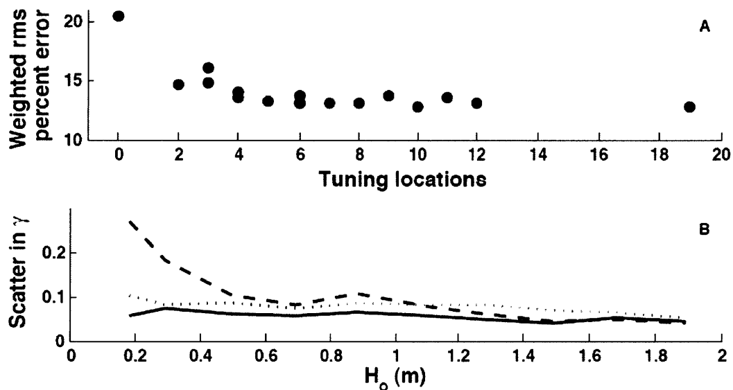
Figure 2-11: (A) Weighted rms percent error versus the number of tuning locations used with the TG model at SandyDuck, and (B) the scatter (defined as one standard deviation of the best-fit \gamma ) of the best-fit \gamma versus the deep-water wave height H_o when the TG model is tuned using data from all sensors (solid curve), 2 offshore sensors and 2 shallow sensors (dashed curve), and 3 shallow sensors, but only 1 offshore sensor (dashed-dotted curve). Tuning locations used in (A) were chosen to span the surfzone for most conditions. For 3, 4, and 6 tuning locations, two different sets of locations were tested (i.e., 2 symbols in the vertical at tuning locations = 3, 4, and 6 in A).
