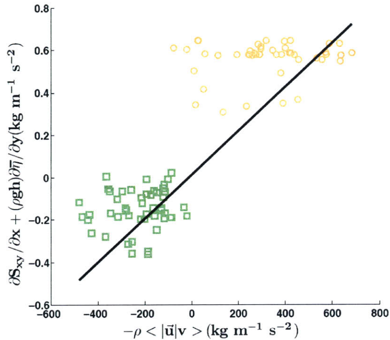
Figure 5-9: The total forcing ( \partial S_{xy}/\partial x + (\rho gh)\partial\bar{\eta}/\partial y ) versus the velocity term ( -\rho \langle \vec{u} | \vec{v} \rangle ) in the bed stress formulation estimated at the 1.0-m isobath sensors for y = 2321 m (green squares) and 1450 m (orange circles). The black line is the least squares fit, and has a slope (i.e., c_d ) of \approx 0.001 . Only data records when the 1.0-m isobath sensor was in the surfzone were used.
