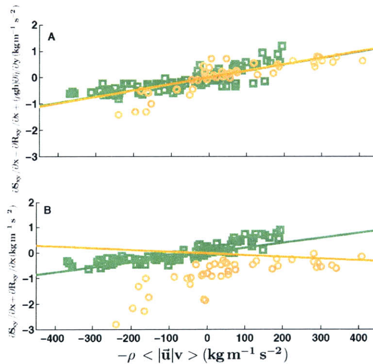
Figure 5-10: (A) The total forcing ( \partial S_{xy} / \partial x + \partial R_{xy} / \partial x + (\rho g h) \partial \bar{\eta} / \partial y ) and (B) the wave and roller-only forcing ( \partial S_{xy} / \partial x + \partial R_{xy} / \partial x ) versus the velocity term ( -\rho \langle \vec{u} | \vec{v} \rangle ) in the bed stress formulation at the 1.0-m isobath sensors for y = 2321 m (green squares) and y = 1450 m (orange circles) when large gradients in H_{rms} on the 2.5-m isobath were observed for 1300 < y < 1450 m. The lines are the least squares fits (forced through 0) of the symbols with the same color.
