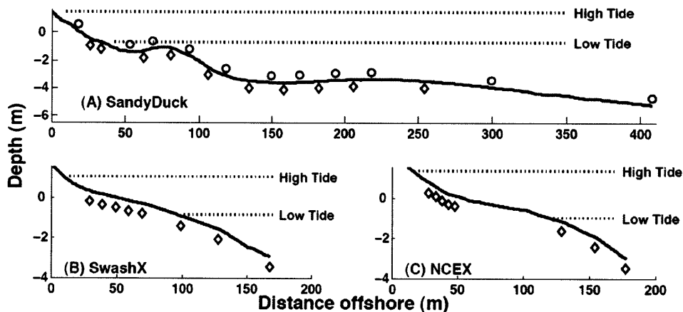
Figure 3-1: Observed bathymetry (solid curves), unburied pressure gages (circles), and buried pressure gages (diamonds) versus distance offshore for SandyDuck (A), SwashX (B), and NCEX (C).
