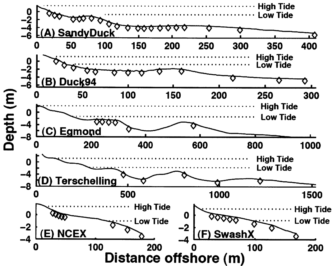
Figure 2-1: Water depth (relative to mean sea level) (solid curves), pressure sensor locations (diamonds), and tidal levels (dotted lines) versus distance offshore for (A) SandyDuck, (B) Duck94, (C) Egmond, (D) Terschelling, (E) NCEX, and (F) SwashX. The most offshore sensors for Egmond (15 m depth) and Terschelling (9 m depth) are not shown.
