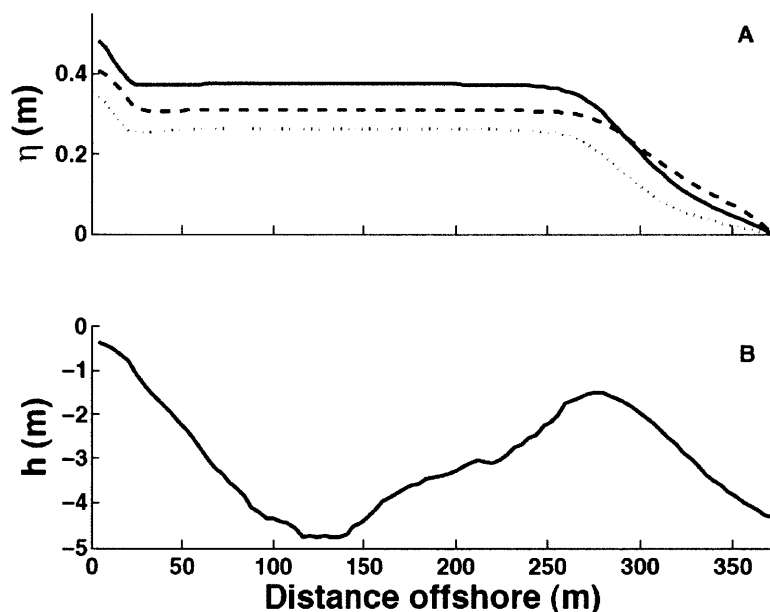
Figure 4-8: (A) Setup simulated using the full model [(4-1) through (4-3), solid curve], the model without the roller term (dashed curve), and the model without the bottom stress term (dotted curve) for (B) the barred beach profile near Egmond, The Netherlands on 18 October, 1998 relative to still water level versus the distance offshore. For this simulation, the offshore wave height was 2.1 m and the still water (tidal) level was -1.7 m relative to MSL.
