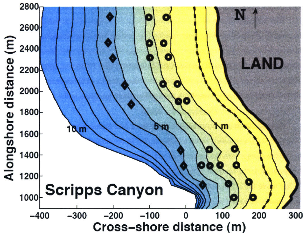
Figure 5-1: Nearshore bathymetry showing the isobaths in 1.0 m intervals (black curves) and the locations of the current meters collocated with buried (circles) and unburied (diamonds) pressure sensors. The dashed curve is the mean sea level shoreline. The bathymetry extends from 2 m above (darkest yellow) to 10 m below (darkest blue) mean sea level. North is approximately at the top of the figure.
