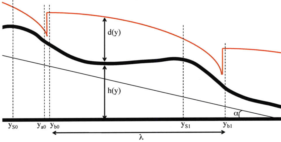
Figure 15: Definition of variables. The thick black line shows the topography, given by the function h(y) . It has overall slope \alpha and spatial period \lambda . The water depth is given by the red line, showing an hydraulic jump after each local topographic maximum.
