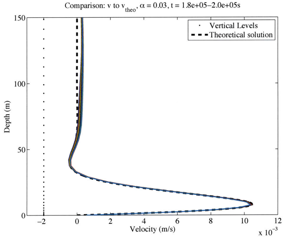
Figure 7: Diffusion Driven Flow over a Constant Slope. The dashed black line indicates the predicted theoretical solution for along-slope velocity, while the colored lines show profiles taken from the numerical solution over the course of several hours. These profiles were taken after more than ten times the adjustment timescale of the boundary layer had elapsed, when the model was at a steady state. The dots on the left side of the plot indicate height of the vertical levels of the grid. The bottom slopes up to the right of the figure.
