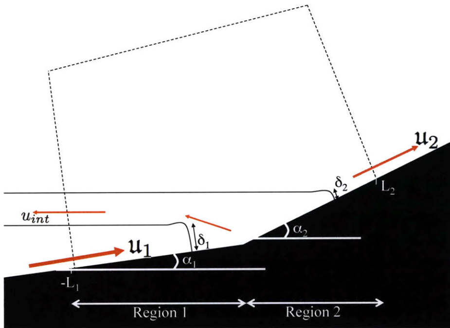
Figure 6: Schematic of dynamics of a diffusion-driven boundary layer over topography with two slopes. In Region 1, the slope has angle \alpha_1 , forcing a velocity u_1 . Similarly, in Region 2, the slope has angle \alpha_2 , forcing a velocity u_2 . Since the total flux in Region 1 is larger than in Region 2, an intrusion is formed as fluid is forced out of the boundary layer, shown by u_{int} . The dashed line shows a hypothetical box that we can use to make mass, volume, and energy budgets.
