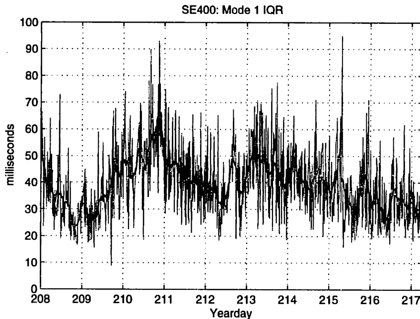
Figure 5-9: Mode 1 IQR for SE400. Gray line is unfiltered IQR, and black line is a 4-hour running average.
