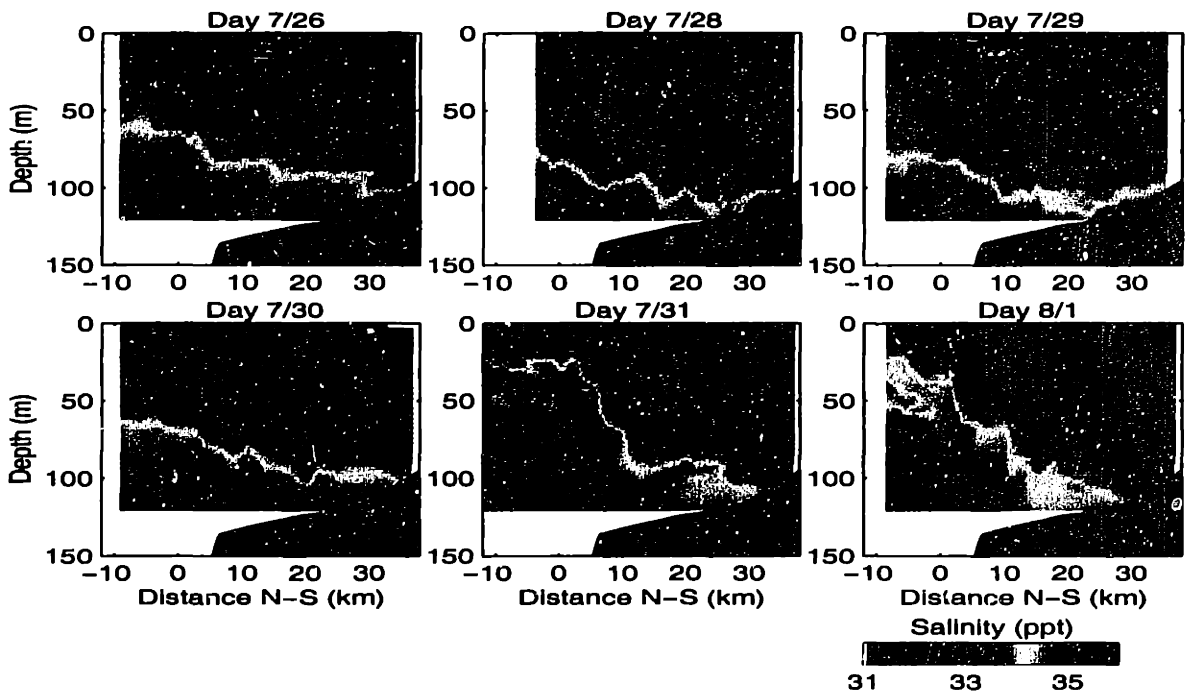
(b) Salinity
