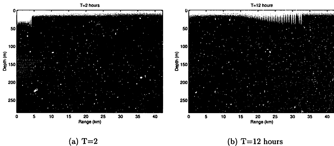
Figure 4-15: Examples of sound speed profiles under perturbation by the solibore field.
