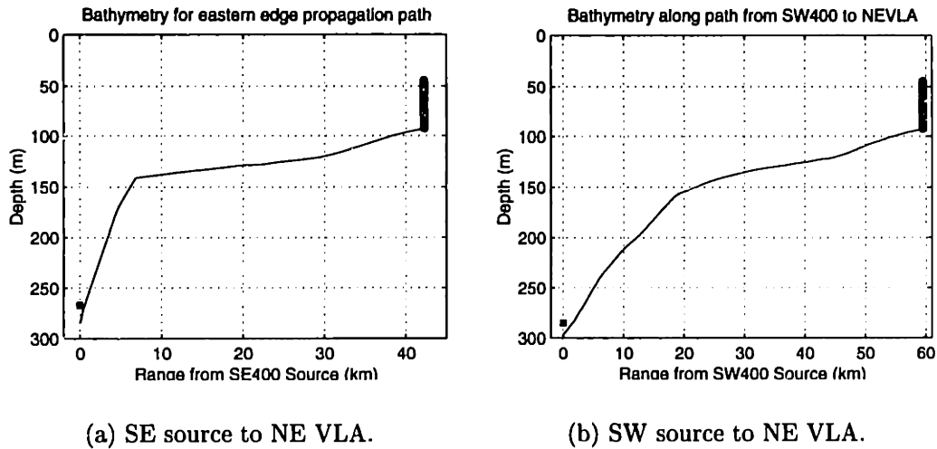
Figure 4-1: Bathymetric sections along acoustic propagation paths.
