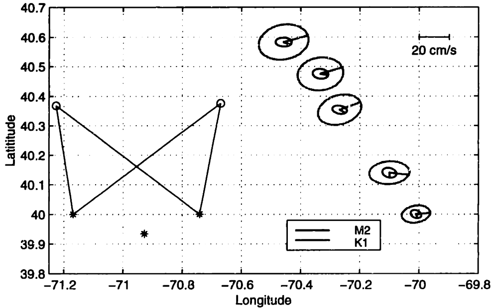
Figure 2-9: Tidal ellipses based on data from moorings along TOPEX/Poseidon subtrack. Tidal phases are indicated for June 27, 1996 00:00GMT. PRIMER acoustic moorings included for reference. (Data provided by Alberto Scotti of WHOI.)
