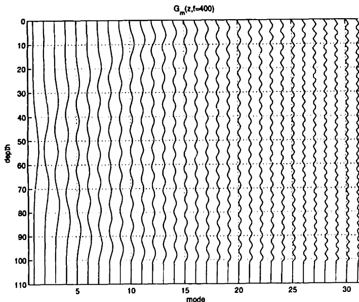
Figure 6-3: Kernel functions.
