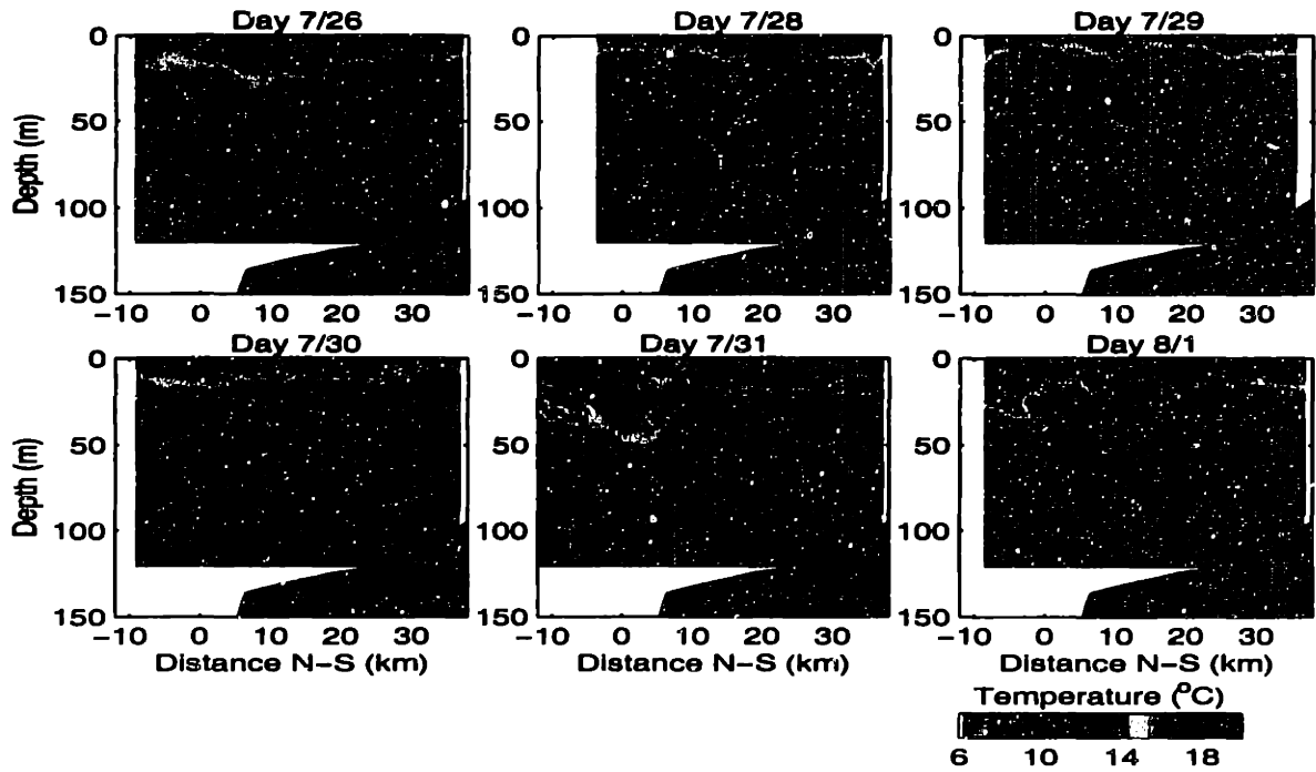
(a) Temperature
